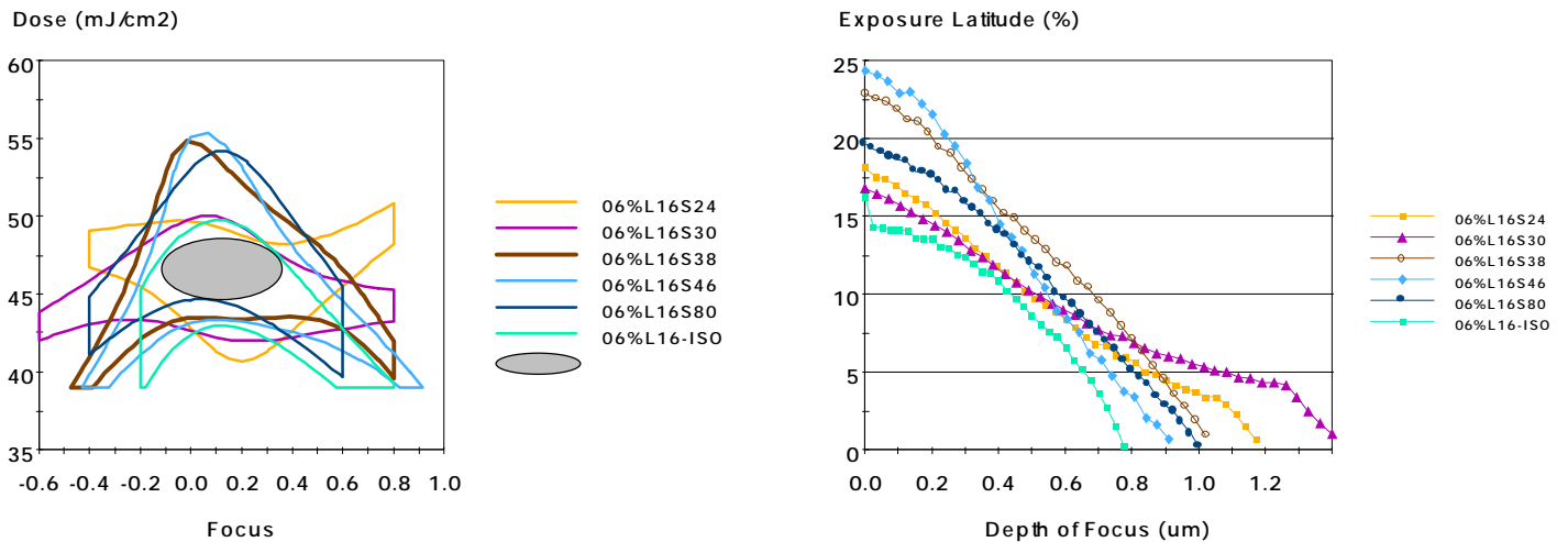
Figure 12: 6% Attenuated mask process window for 1:1.5, 1:2, 1:2.5, 1:3, 1:5 and isolated features with high contrast resist and conventional illumination 0.6NA, 0.8σ
