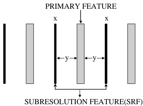
Figure 3: Schematic showing the subresolution feature of size x nm
